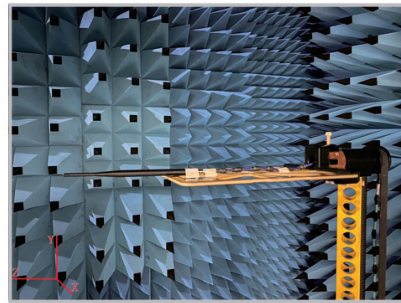
Test Chamber
